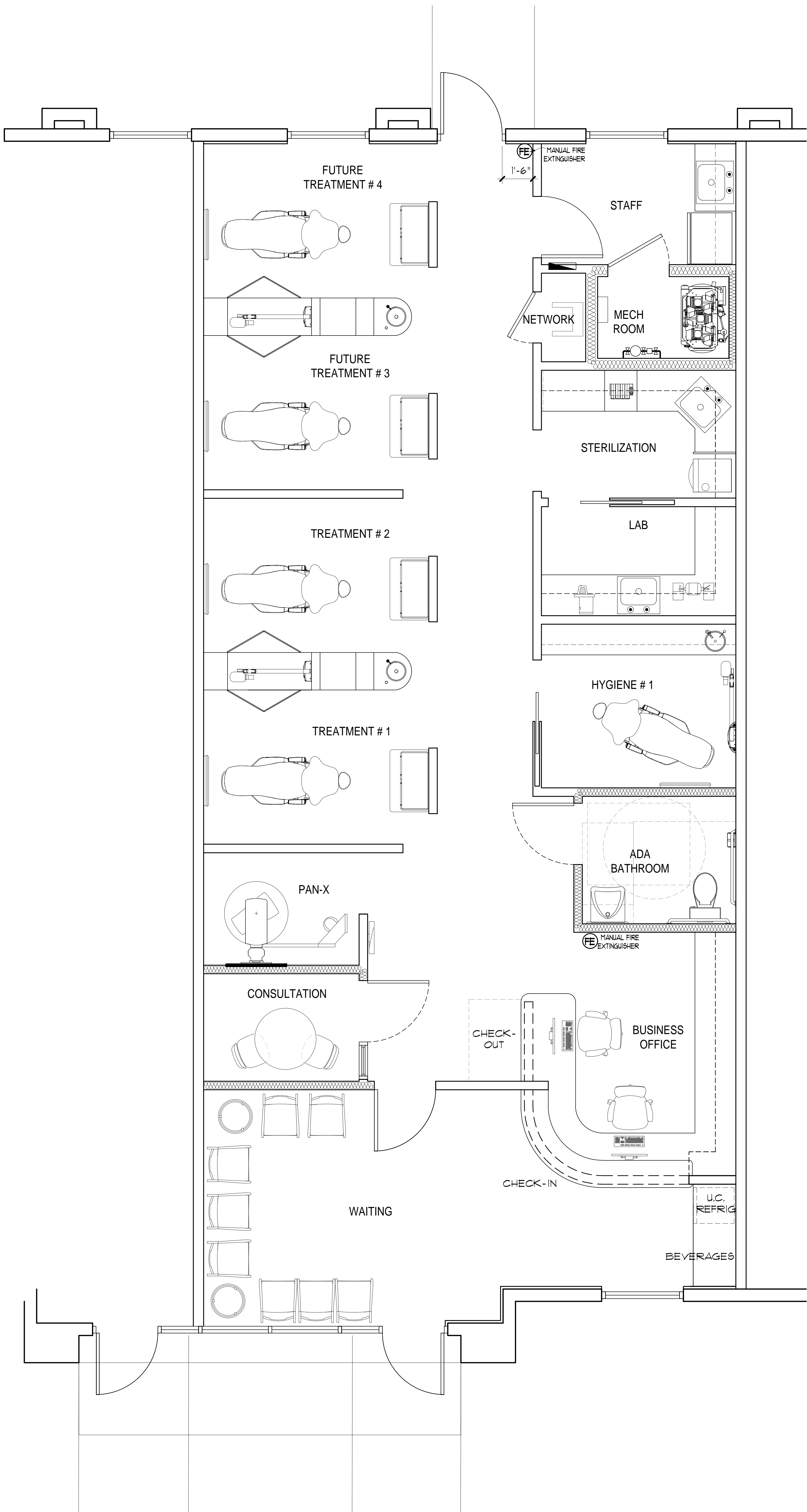
DENVEST DELRAY ATLANTIC & 441 General Dentist Floor Plan
