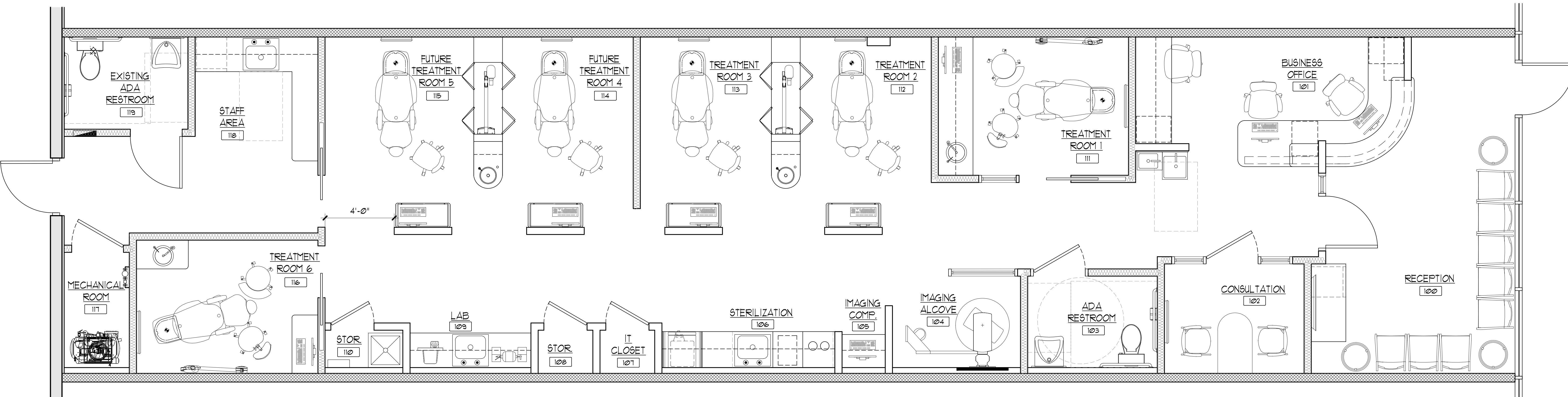
Den-Vest Dental Pompano Beach Floor Plan
